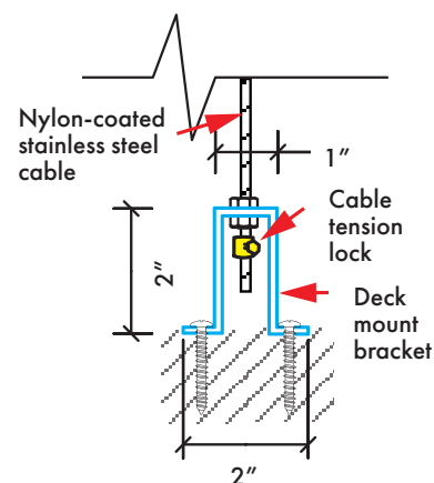
Deck mount cable bracket
