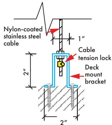
Deck mount cable bracket
