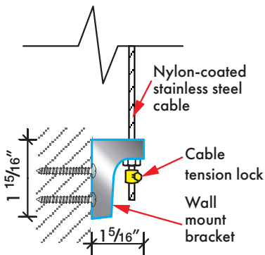
Wall mount cable bracket
